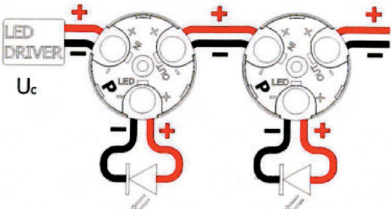
L539406P Verteilerbox Parallel / L539406P Distribution Box - Parallel
